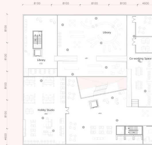
3F Plan
