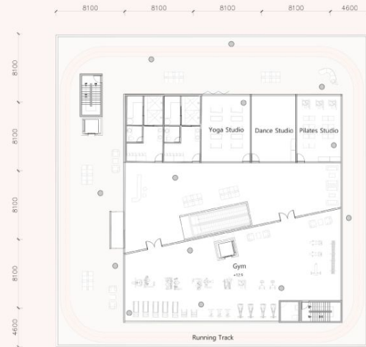
4F Plan
